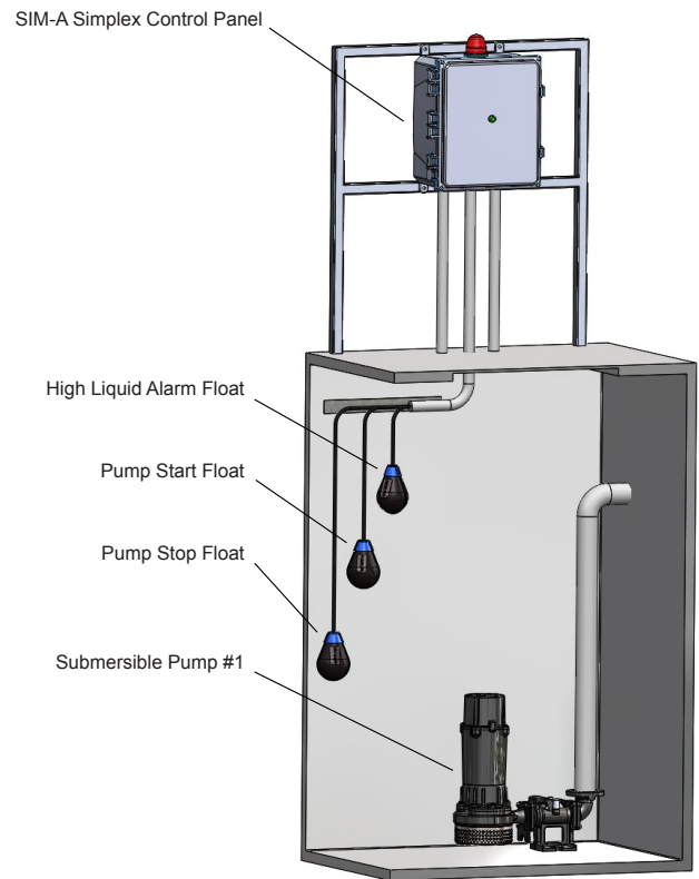
Typical Installation of SIM-A Simplex Control Panel
